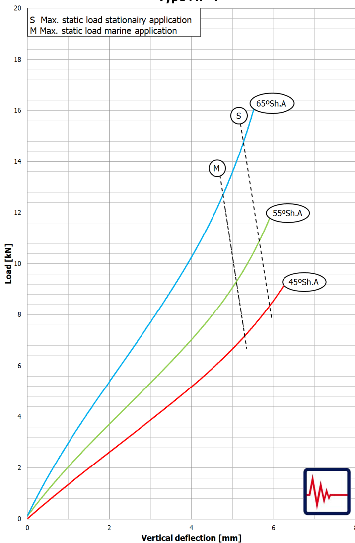
Vertical load / deflection characteristics Type MP-4
