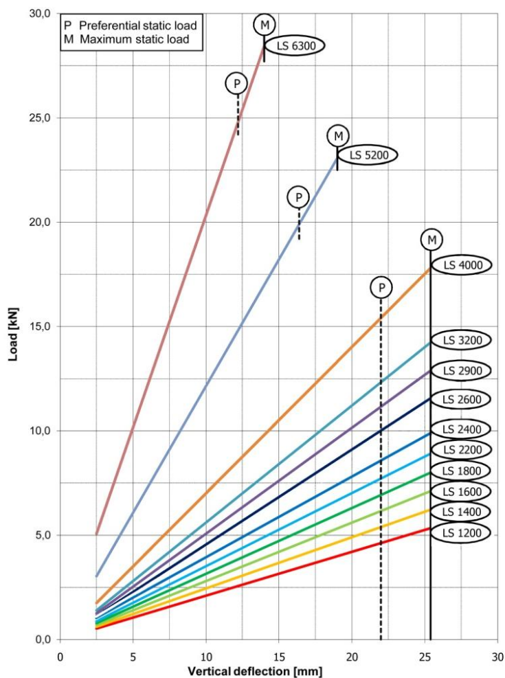
Vertical load / deflection characteristics LS
