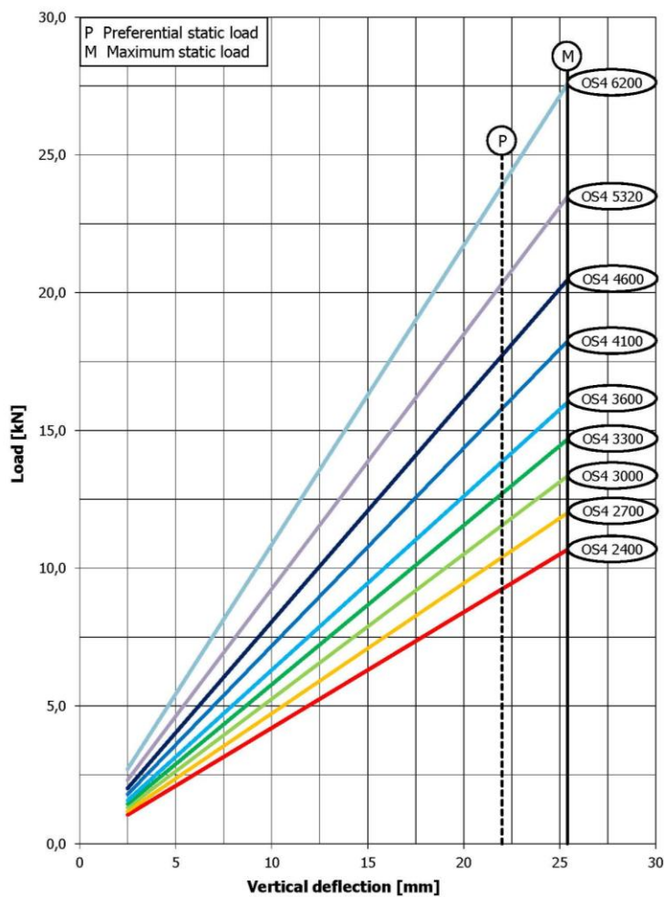
Vertical load / deflection characteristics OS4
