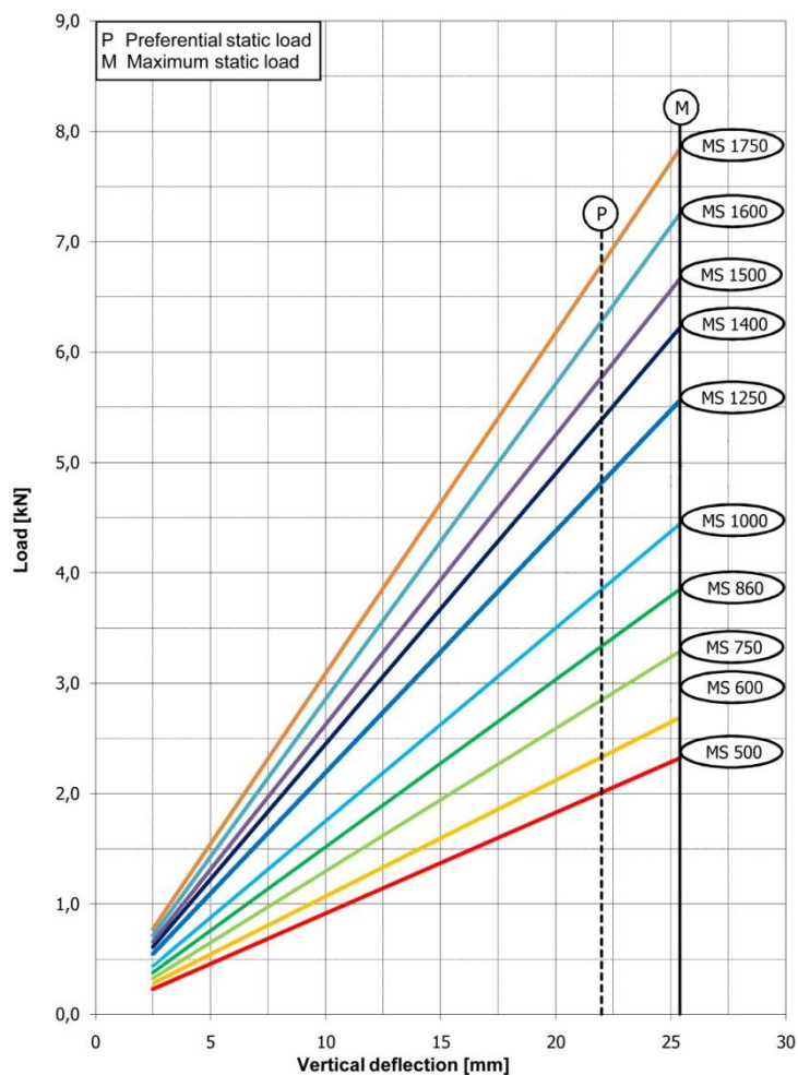
Vertical load / deflection characteristics MS
