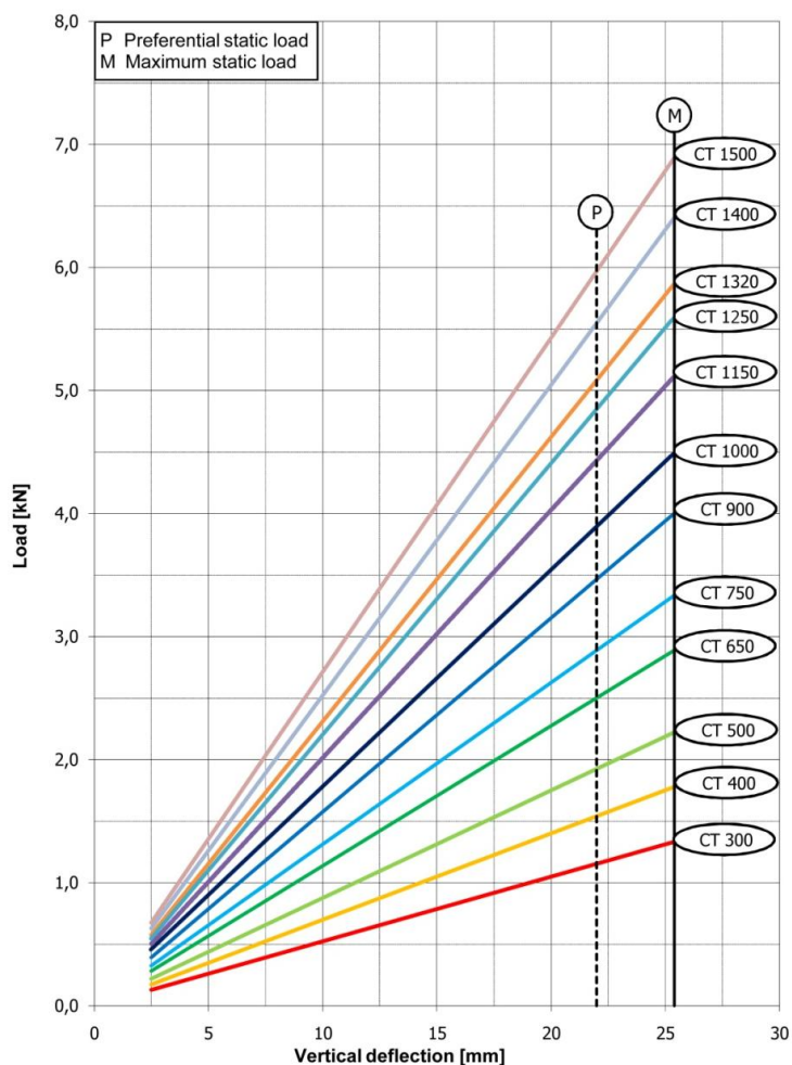
Vertical load / deflection characteristics CT
