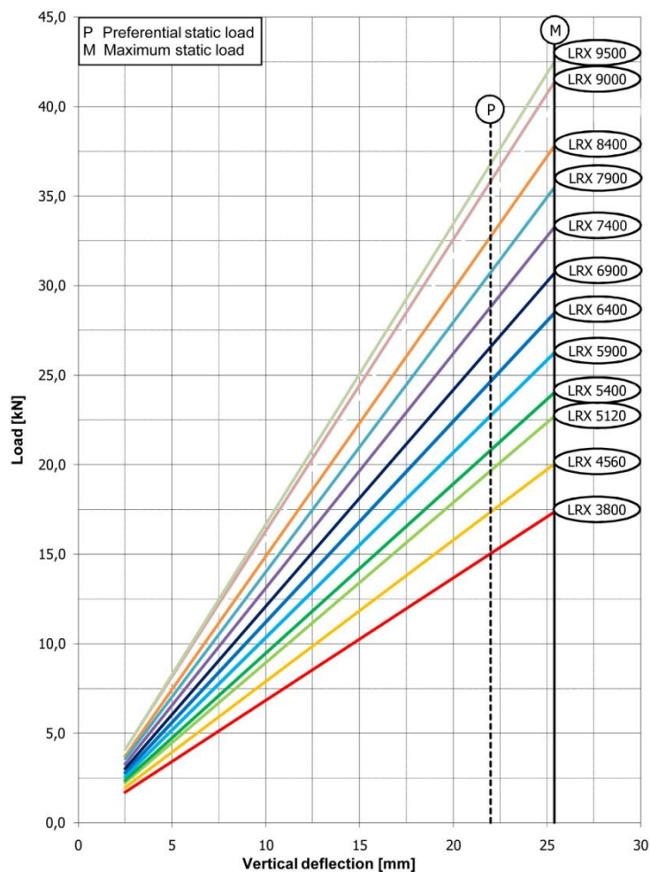
Vertical load / deflection characteristics LRX
