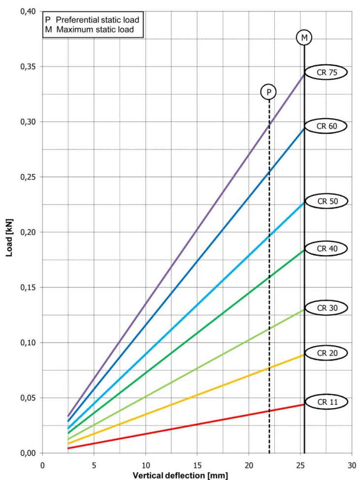
Vertical load / deflection characteristics CR
