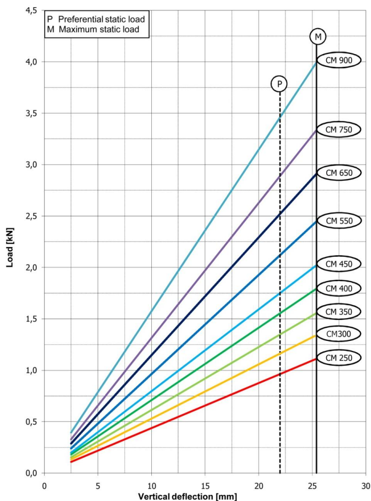
Vertical load / deflection characteristics CM
