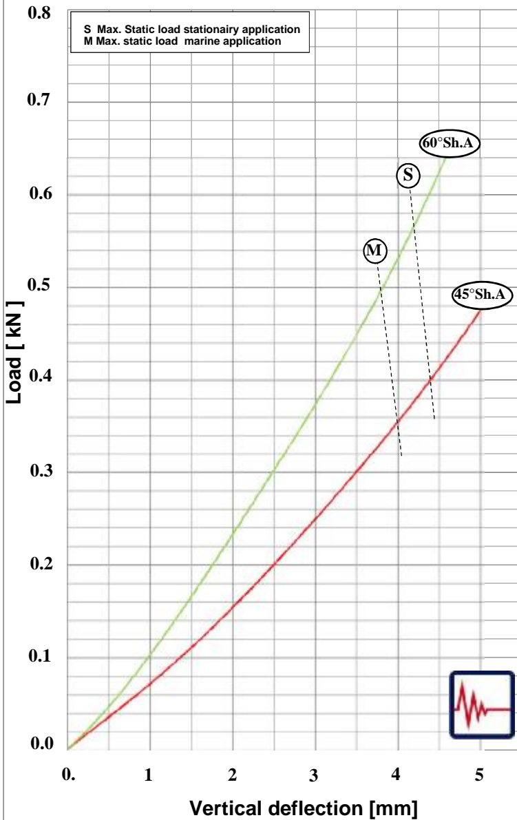
Vertical Load / deflection Characteristics Type MP-1
